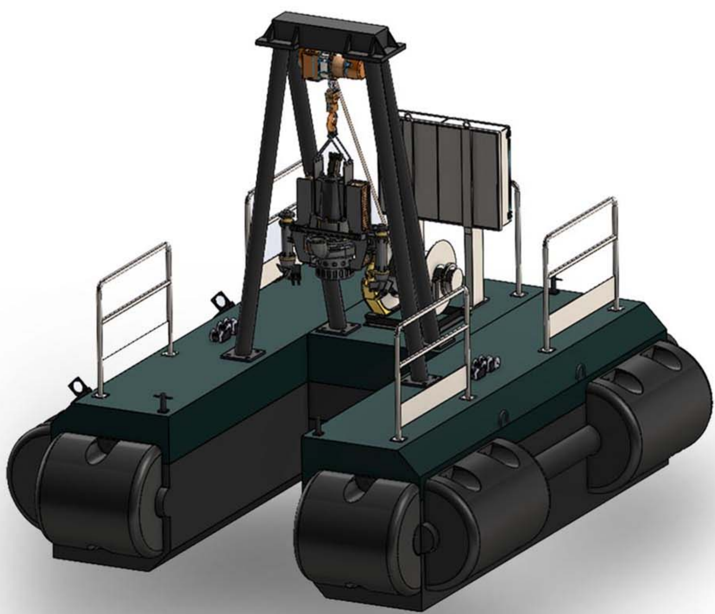
Gordon Pontoon series, solusi pemompaan offshore
